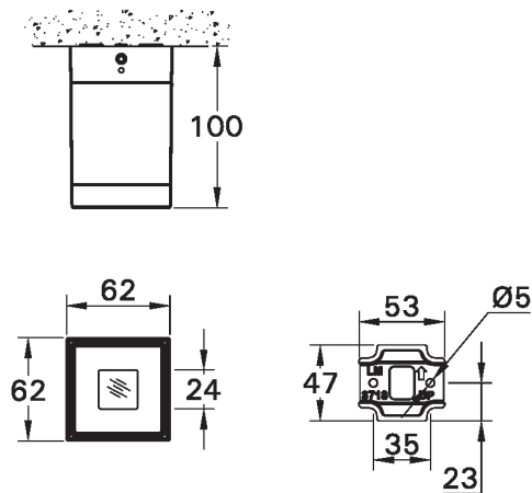
MOUNTING DETAIL
